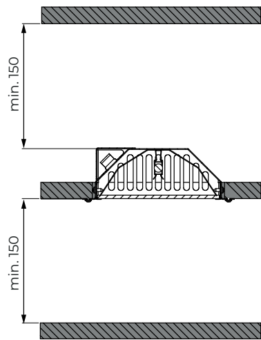
Safety distances for Sentio by Harvia infrared radiators (DIR-750-R)
