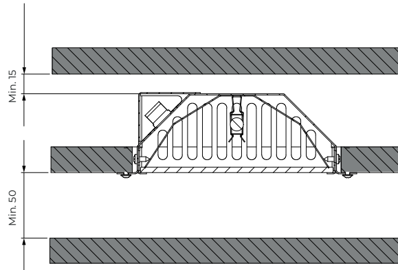
Safety distances for Sentio by Harvia infrared radiators (DIR-350-R, DIR-350-R-F, DIR-500-R, DIR-500-R-F)
