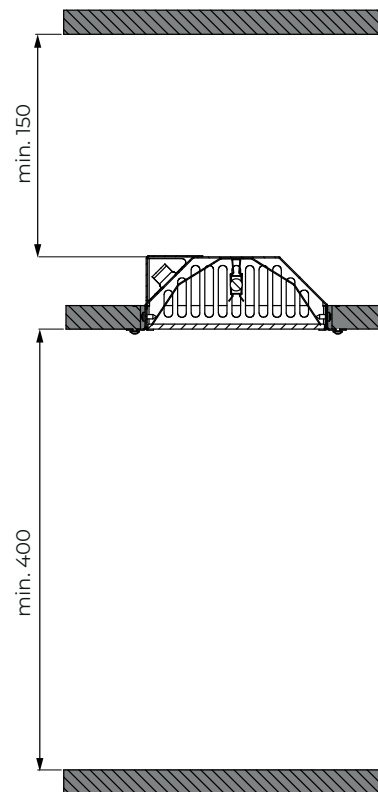
Safety distances for Sentio by Harvia infrared radiators (DIR-1300-R)
